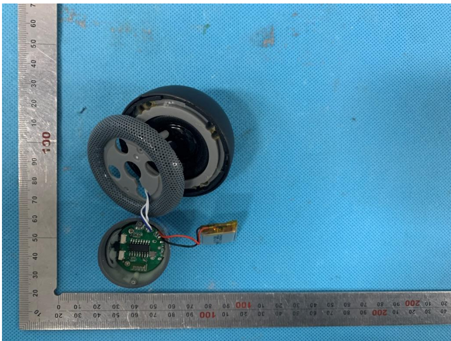
Fig.4 – open view
