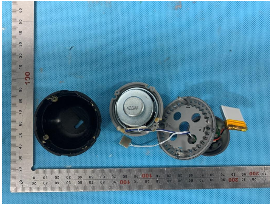
Fig.5 – open view
