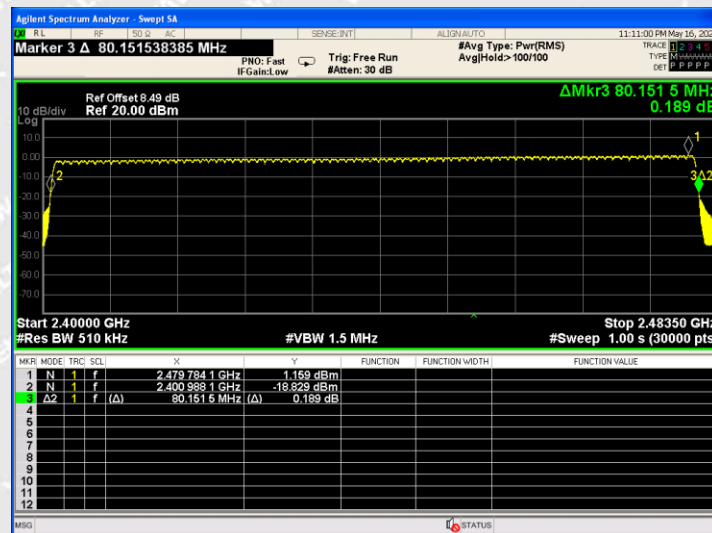
Hopping Sequence_2DH5
