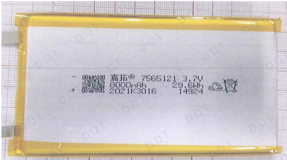
Fig. 11 – Battery view
