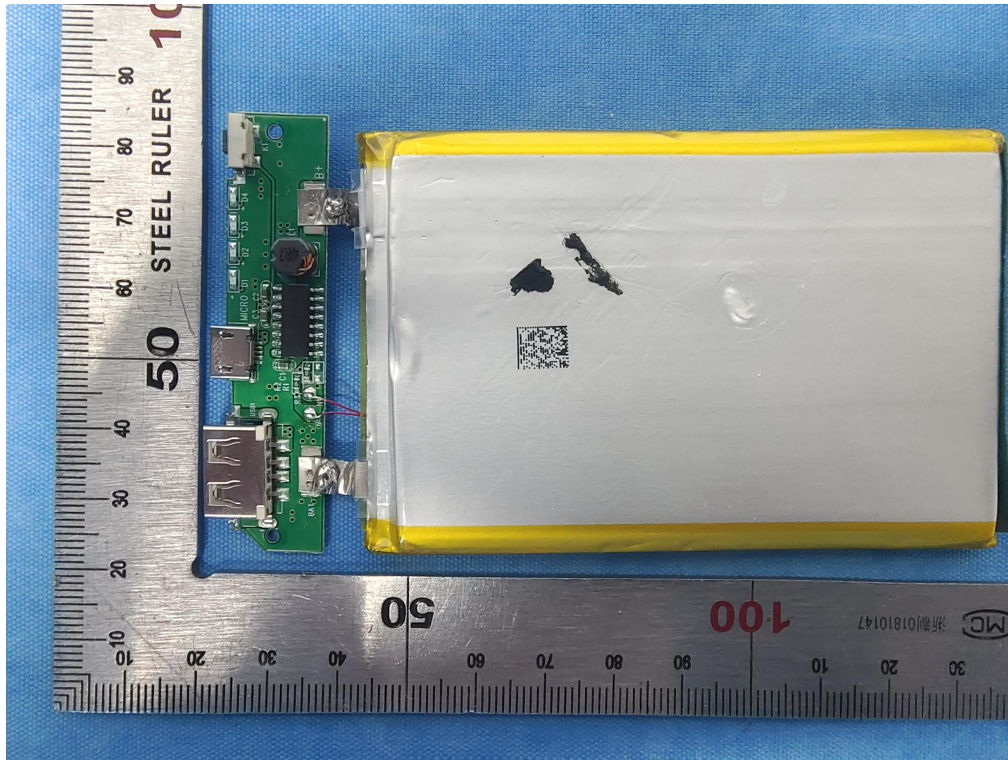
Fig. 5 –Battery view
