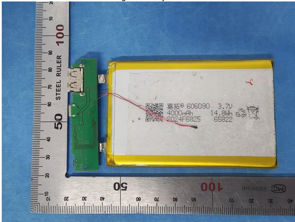
Fig. 6 –Battery view
