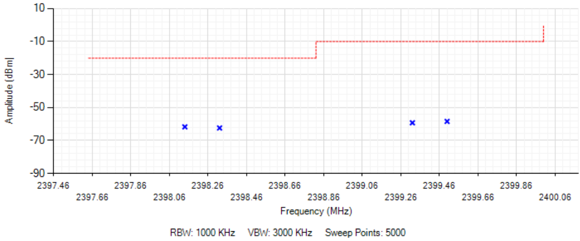
Transmitter unwanted emissions in the out-of-band domain
