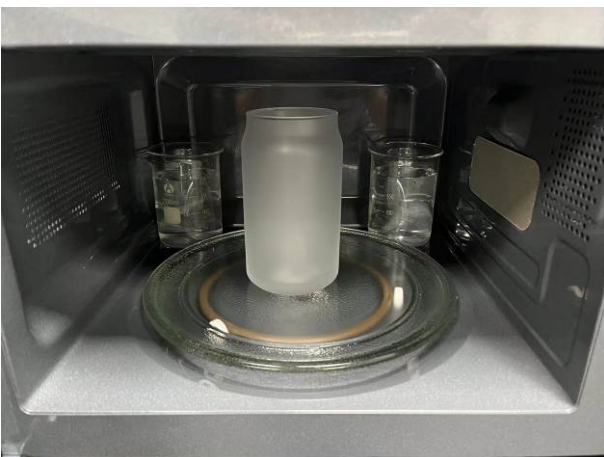
2#-During Testing
