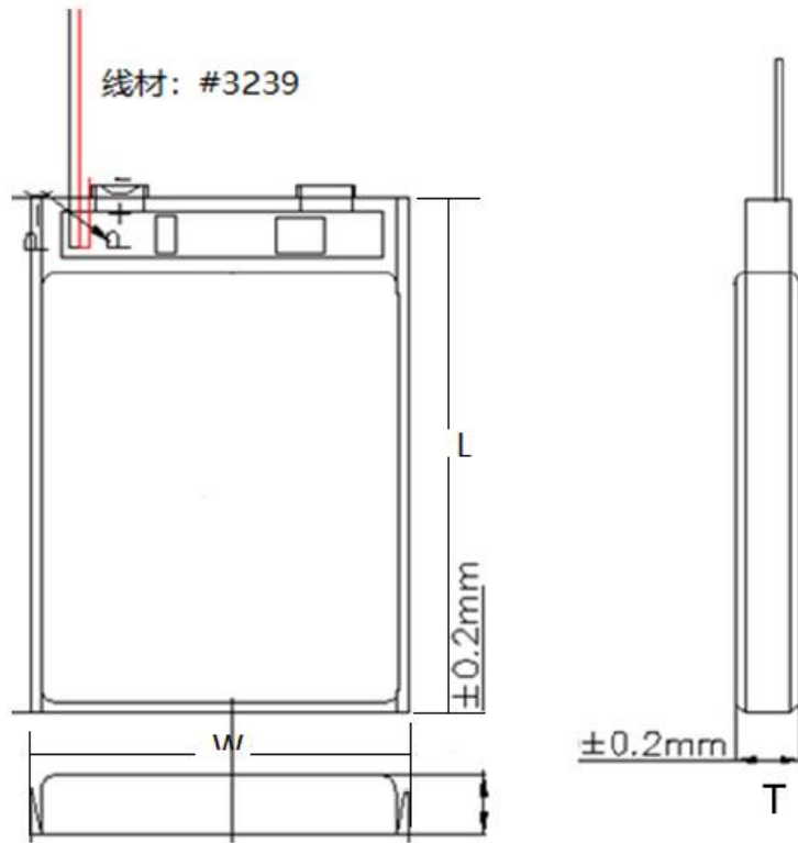
T*W*L=6.0\text{ (max)}*20.0\text{ (max)}*30.0\text{ (max)} Battery (Unit: mm)
