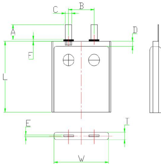
T*W*L=6.0 (max)*20.0 (max)*30.0 (max) Cell (Unit: mm)
