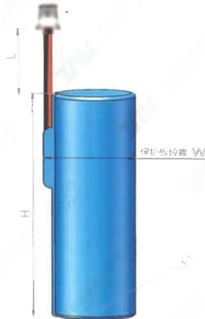
\phi * H = 19.0 (max) * 67.0 (max) Battery (Unit: mm)
