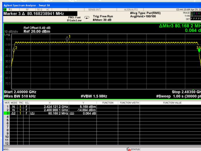
Hopping Sequence_2DH5
