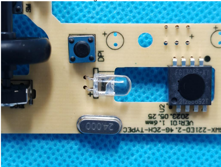
Fig.2- LED light view
