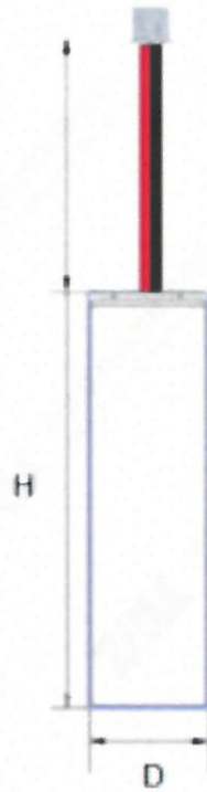
D*H=16.3 (max)*51.1 (max) Battery (Unit: mm)
