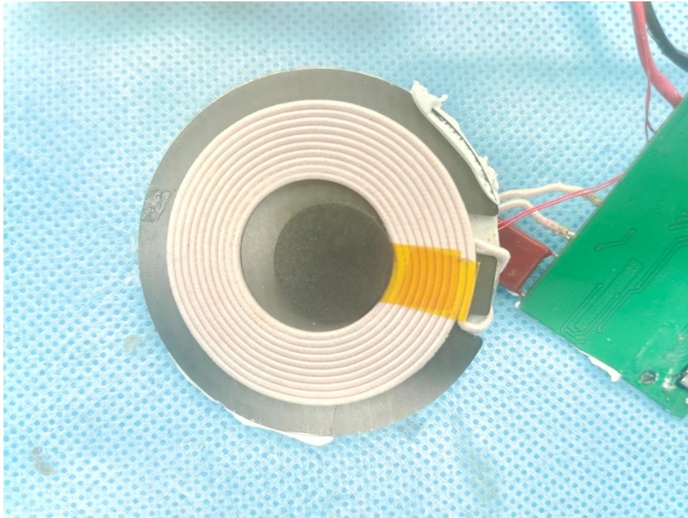
Fig.9 – Part view
