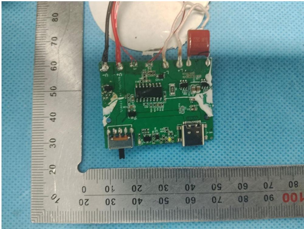
Fig.6 – part view
