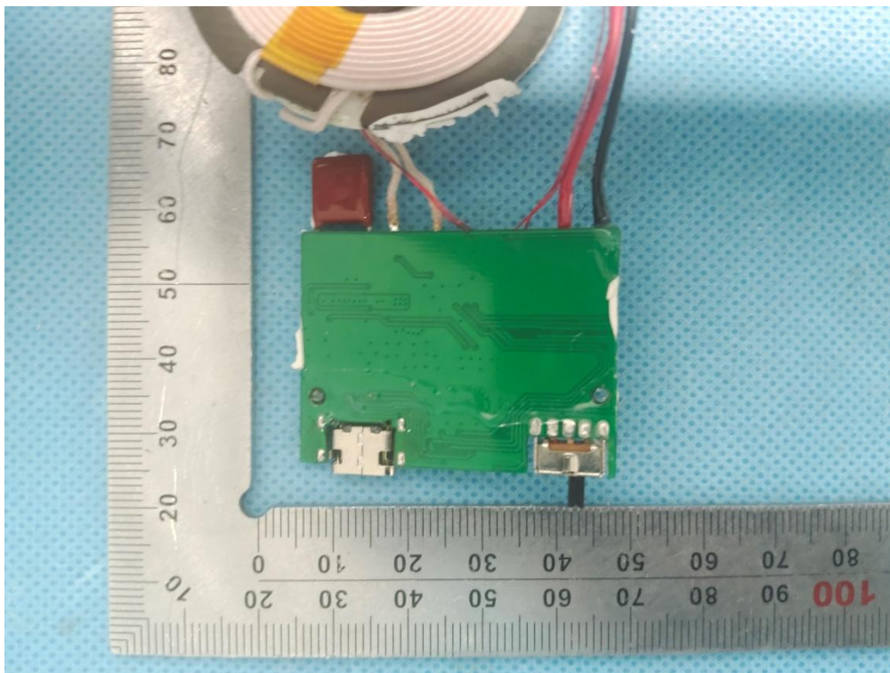
Fig.8 – Part view
