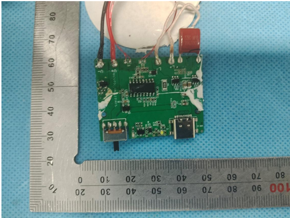
Fig.7 – Part view
