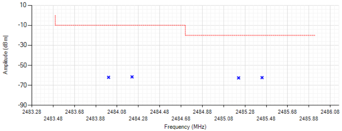
Transmitter unwanted emissions in the out-of-band domain
