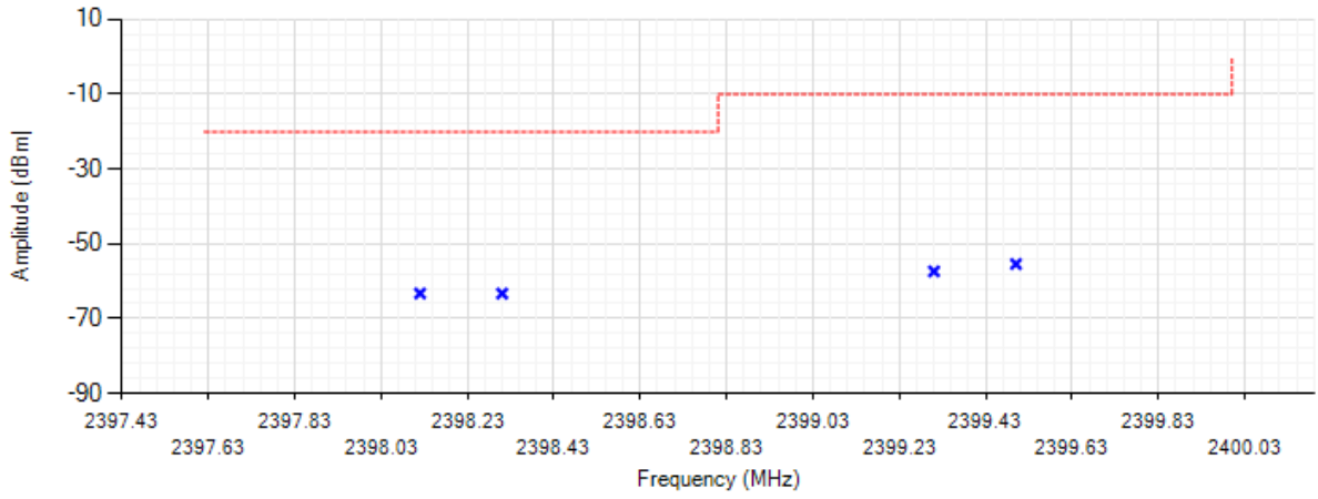
Transmitter unwanted emissions in the out-of-band domain
